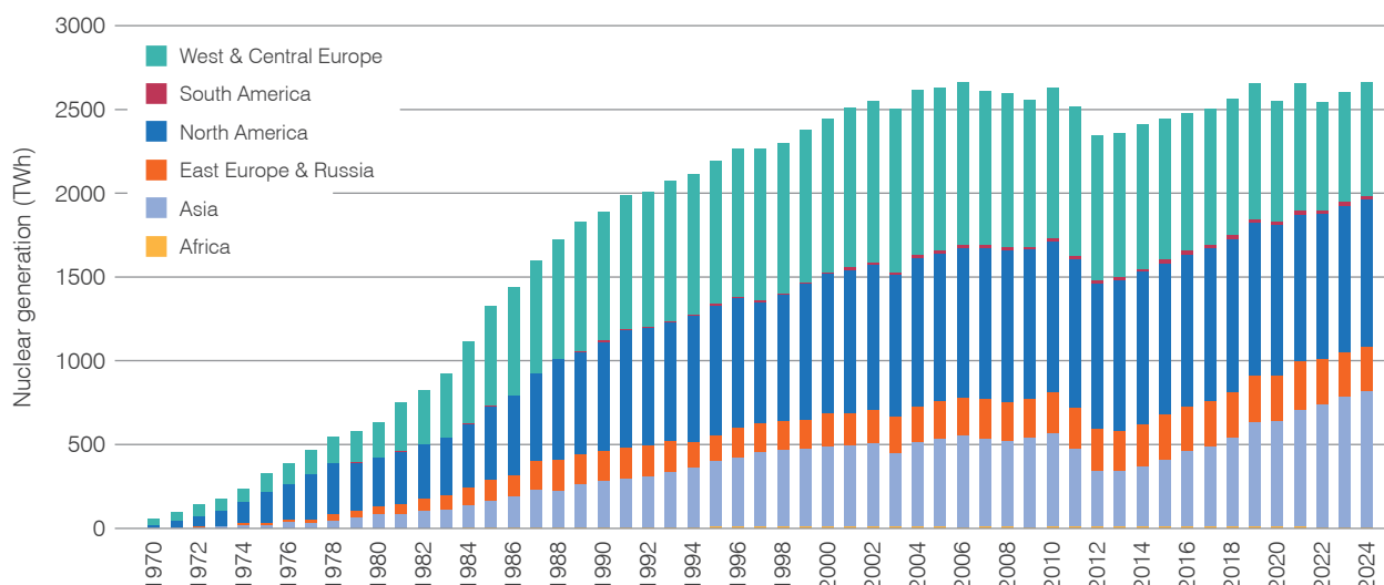
Figure 1.1 Global nuclear generation by region
